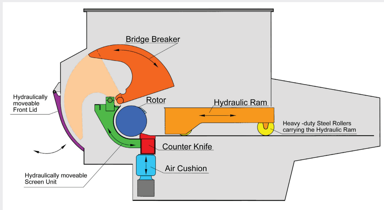
Illustrations of the operation of the BridgeBreaker and "Flipper" Floating Counter Knife
