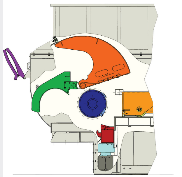
Illustrations of the operation of the BridgeBreaker and "Flipper" Floating Counter Knife
