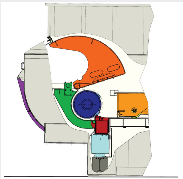
Illustrations of the operation of the BridgeBreaker and "Flipper" Floating Counter Knife
